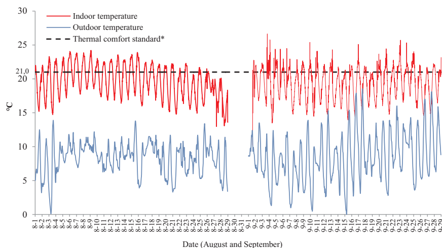
Fig. 7. Indoor (40-house average) and outdoor temperatures in August and September 2017. *WHO recommends 21 °C in the living room and 18 °C in the rest of the house (WHO, 1987).
